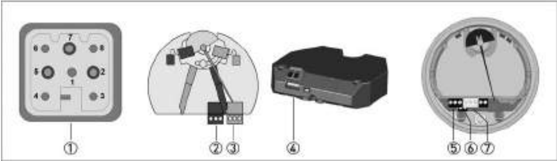
① Terminal pin assignment HAN® 7D - View of plug connection
