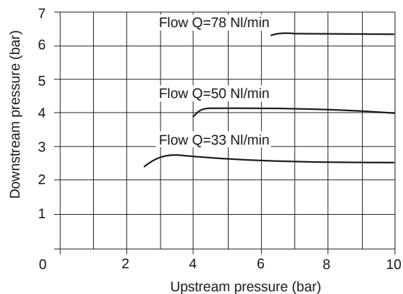
Adjustment characteristics
